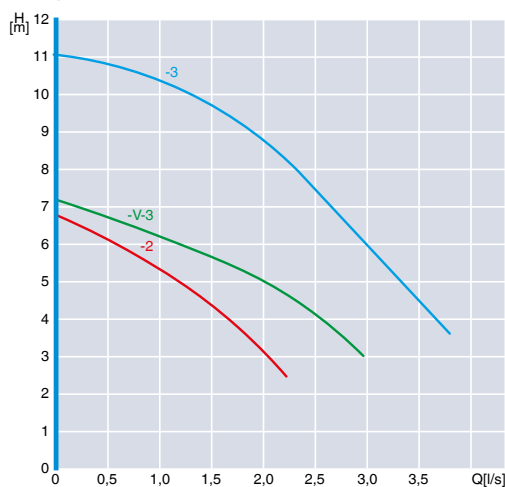
Pumpekurve model SX
